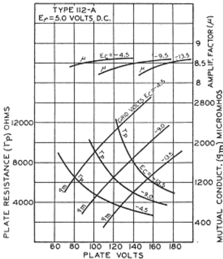
AVERAGE CHARACTERISTICS
